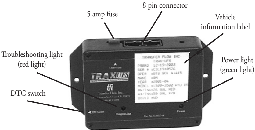
Trax-UFS Computer Module FIGURE 2
