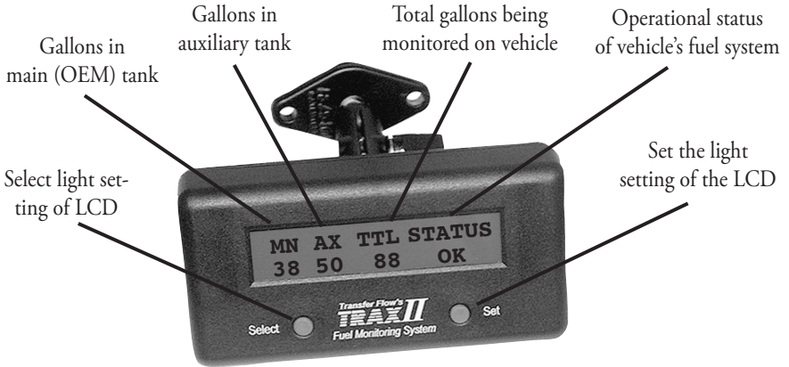
Dash Mounted LCD FIGURE 1
